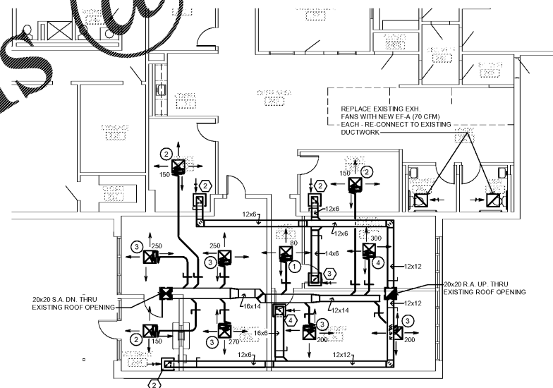
PARTIAL HVAC FLOOR PLAN - EXISTING BUILDING SCALE: 1/8" = 1'-0"
