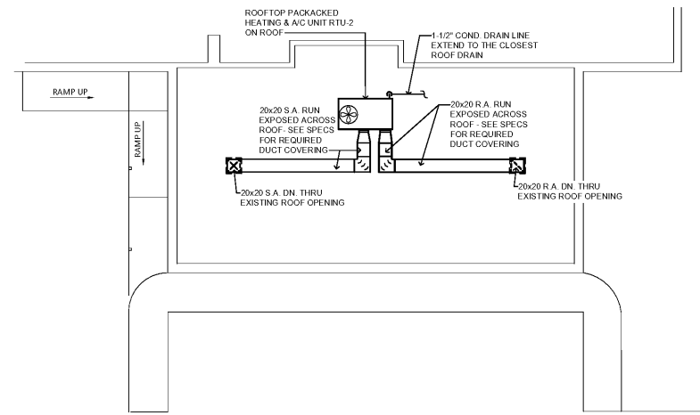
PARTIAL HVAC ROOF PLAN - EXISTING BUILDING SCALE: 1/8" = 1'-0"
