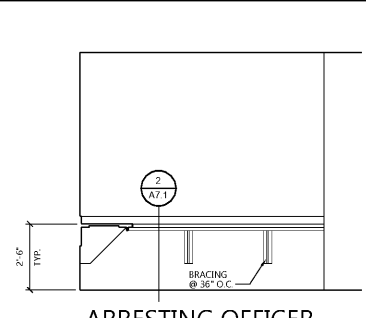
D ARRESTING OFFICER WORKROOM 1351 SCALE: 3/8" = 1'-0"
