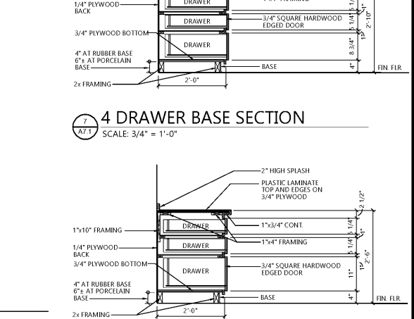
8 3 DRAWER BASE SECTION SCALE: 3/4" = 1'-0"
