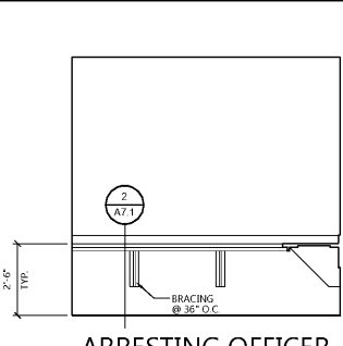
C ARRESTING OFFICER WORKROOM 1351 SCALE: 3/8" = 1'-0"
