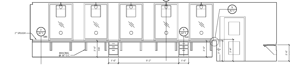
H BOOKING DESK AT PROCESSING 1363 SCALE: 3/8" = 1'-0"
