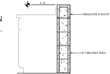
P HALF WALL SECTION at COPIER SCALE: 1" = 1'-0"
