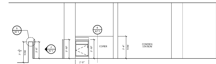
L BOOKING DESK AT PROCESSING 1369 SCALE: 3/8" = 1'-0"
