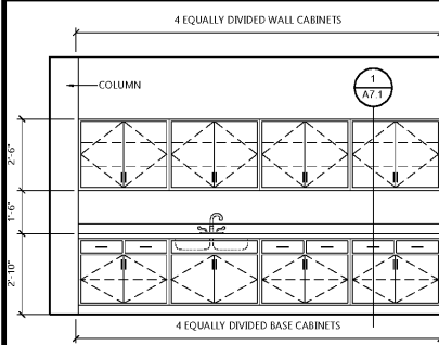
A MEDICAL TRIAGE 1364 SCALE: 3/8" = 1'-0"
