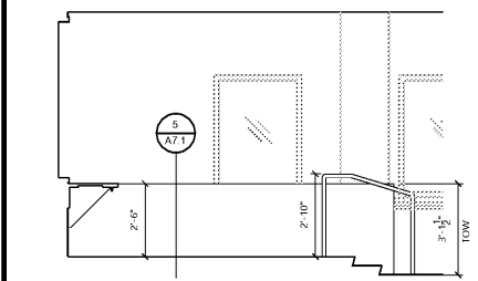
K BOOKING DESK AT PROCESSING 1369 SCALE: 3/8" = 1'-0"
