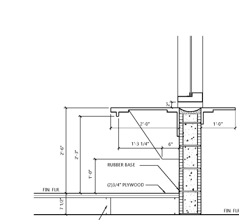
3 PROCESSING WINDOW SECTION SCALE: 1" = 1'-0"
