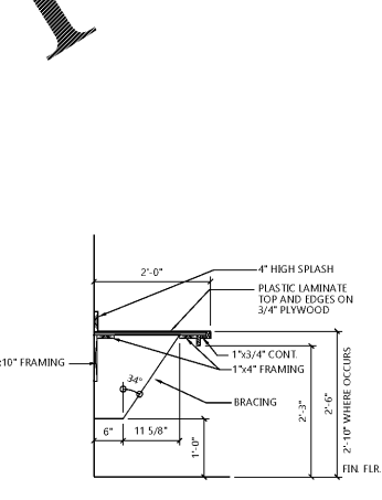
2 COUNTER TOP SECTION SCALE: 3/4" = 1'-0"
