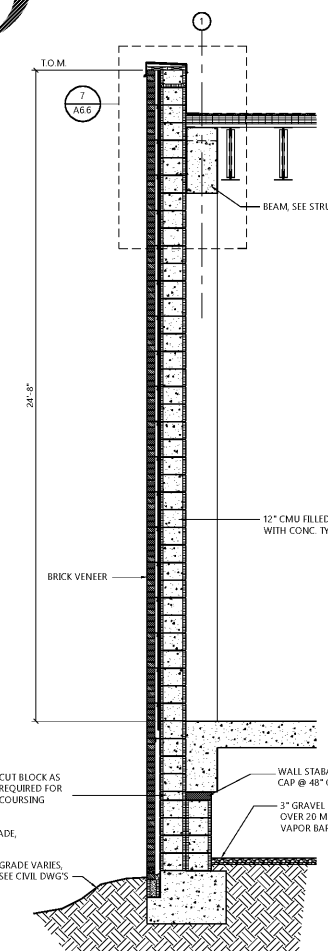
END WALL SECTION at SALLYPORT SCALE: 3/8" = 1'-0"
