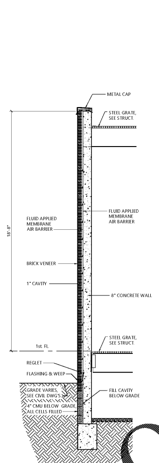
MECHANICAL YARD WALL SCALE: 3/8" = 1'-0"
