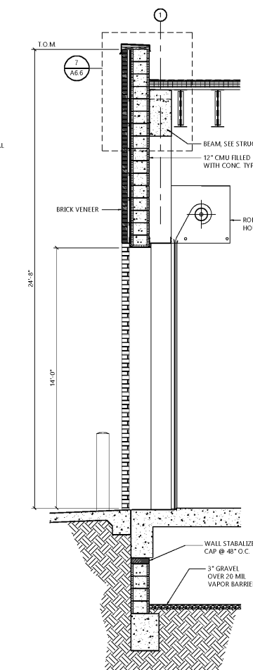
ROLL-UP DOOR SECTION at SALLYPORT SCALE: 3/8" = 1'-0"
