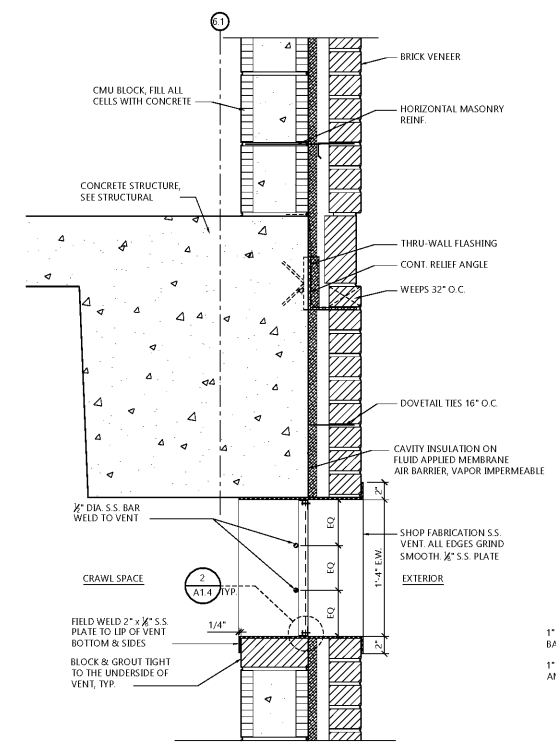
1 TYPICAL CRAWL SPACE VENT DETAIL SCALE: 1 1/2" = 1'-0"
