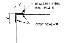
5 A4.1 TYPICAL INSIDE CORNER DETAIL SCALE: 1-1/2"=1'-0"
