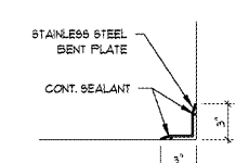
4 A4.1 TYPICAL OUTSIDE CORNER DETAIL SCALE: 1-1/2"=1'-0"
