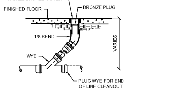
6 FLOOR CLEANOUT DETAIL
