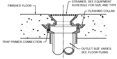
4 FLOOR DRAIN DETAIL
