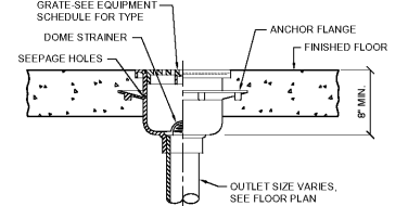
5 FLOOR SINK DETAIL
