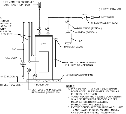
1 DOMESTIC WATER HEATER DETAIL
