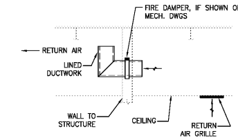
3 RETURN AIR BOOT DETAIL
