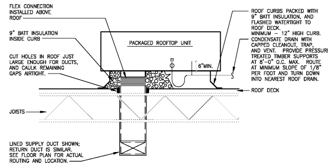
1 ROOFTOP UNIT DETAIL
