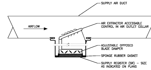
4 REGISTER CONNECTION DETAIL
