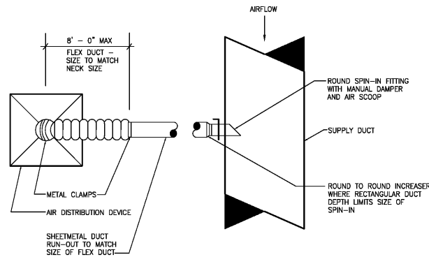
5 DIFFUSER CONNECTION DETAIL
