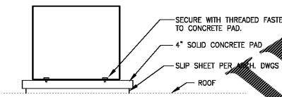
6 CONDENSING UNIT DETAIL
