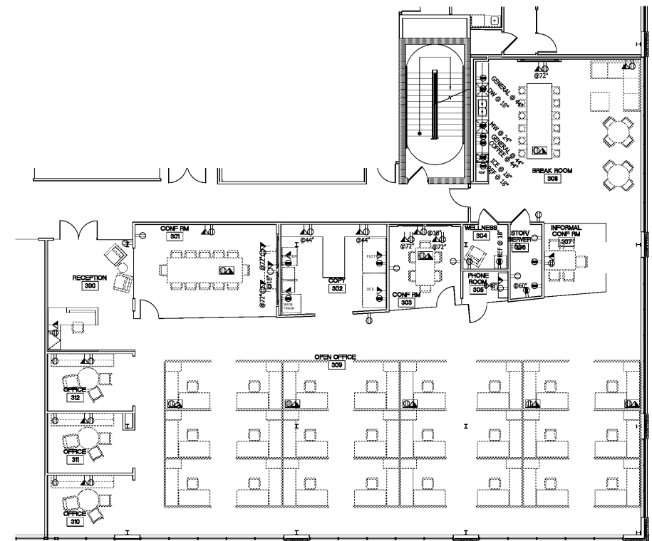
1 FURNITURE PLAN (ELEC FOR REF ONLY) SCALE: 1/8"=1'-0"
