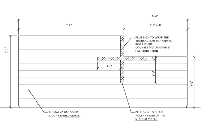
1 ELEVATION @ RECEPTION DESK CUSTOMER SIDE SCALE: 1"=1'-0"
