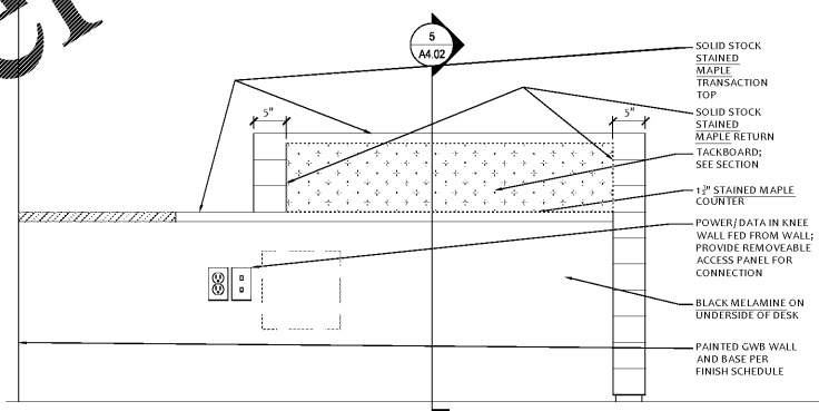
3 ELEVATION @ RECEPTION DESK EMPLOYEE SIDE SCALE: 1"=1'-0"
