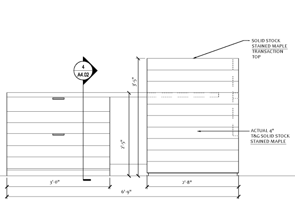
2 ELEVATION @ RECEPTION DESK END SCALE: 1"=1'-0"
