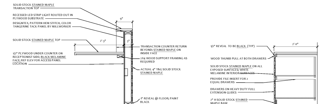
5 SECTION @ RECEPTION DESK SCALE: 1"=1'-0"
