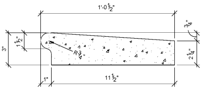
2 PRECAST CONC. COPING STONE 3" = 1'-0"
