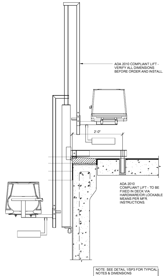
1 ADA COMPLIANT LIFT SECTION 1" = 1'-0"
