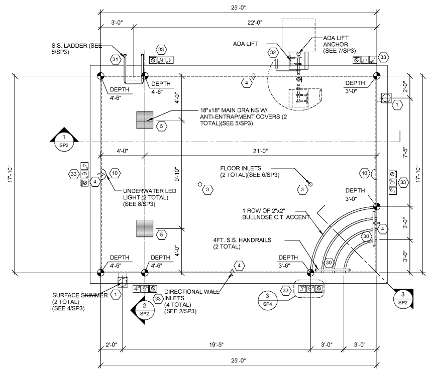
1 POOL PLAN 1/4" = 1'-0"
