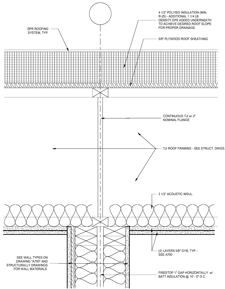
1 FIRESTOPPING/DRAFTSTOPPING @ ROOF 3" = 1'-0"
