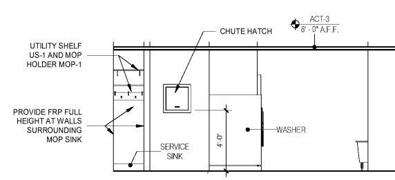
3 LAUNDRY ROOM CHUTE 1/4" = 1'-0"
