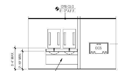
23 PUBLIC RESTROOM - WOMEN MEN'S ROOM REVERSED 1/4" = 1'-0"
