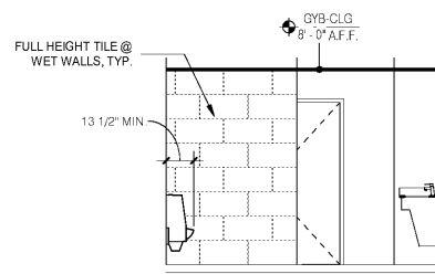
14 PUBLIC RESTROOM - MEN B 1/4" = 1'-0"
