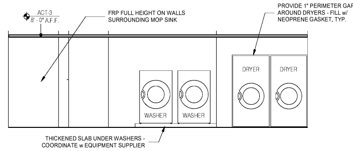
1 LAUNDRY ROOM EQUIPMENT 1/4" = 1'-0"
