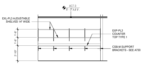
2 LAUNDRY ROOM FOLDING COUNTER 1/4" = 1'-0"
