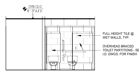
21 PUBLIC RESTROOM - WOMEN B 1/4" = 1'-0"
