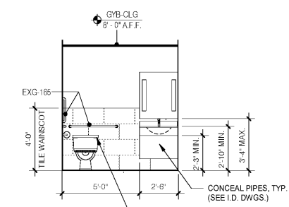
27 POOL UNISEX - A 1/4" = 1'-0"
