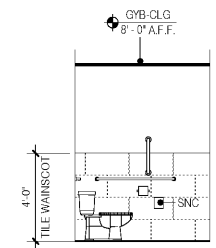
18 EMPLOYEE UNISEX - B 1/4" = 1'-0"
