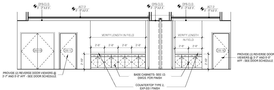
16 CONFERENCE ROOM - CASEWORK WALL 1/4" = 1'-0"
