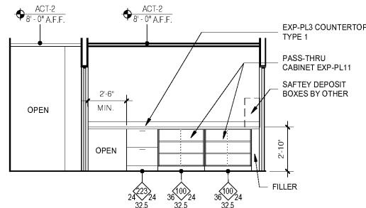
5 WORK AREA CASEWORK 1/4" = 1'-0"
