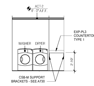
26 GUEST LAUNDRY 1/4" = 1'-0"
