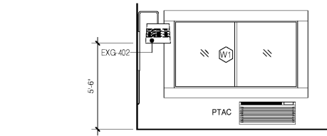
7 QQ - WINDOW 1/4" = 1'-0"
