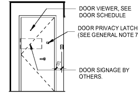
10 QQ - ENTRY - DOOR 1/4" = 1'-0"
