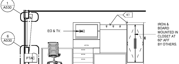
4 QQ - RACK 1/4" = 1'-0"
