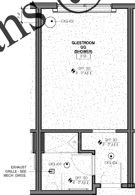
2 GUESTROOM - QQ - RCP 1/4" = 1'-0"
