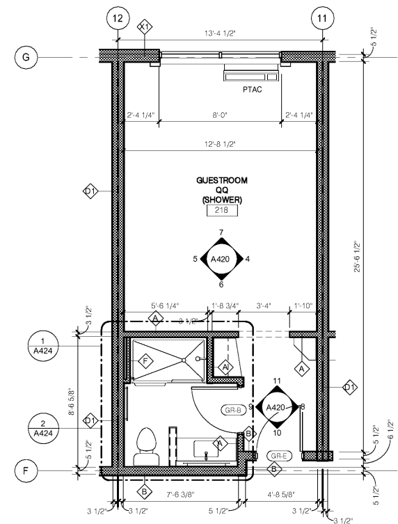
1 GUESTROOM - QQ 1/4" = 1'-0"
