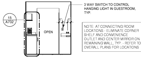
11 QQ - ENTRY - DOOR OPENING 1/4" = 1'-0"
