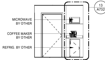
9 QQ - ENTRY - REFRESHMENTS 1/4" = 1'-0"
