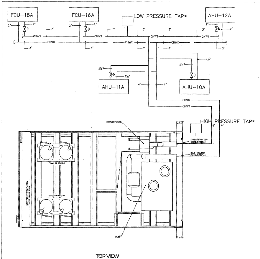
7 CHILLED WATER FLOW DIAGRAM (TYPICAL) M303 SCALE: N.T.S.
