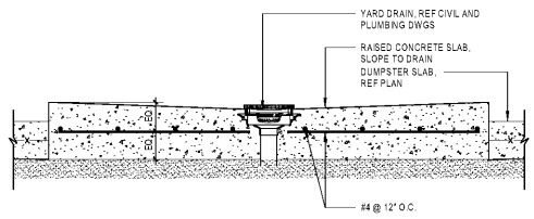
D1 TYPICAL AT DUMPSTER DRAIN 3/4" x 1'-0"
