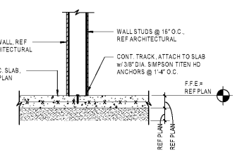
C5 TYPICAL AT INTERIOR NON-LOAD BEARING WALL 3/4" x 1'-0"
