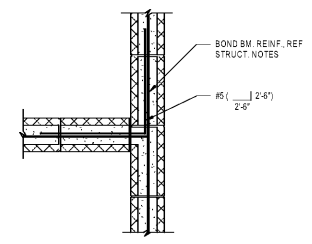
D3 TYPICAL AT 8" KNOCK-OUT BOND BEAM INTERSECTION 3/4" x 1'-0"
