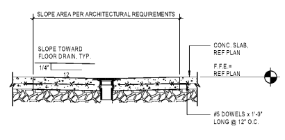
S5 TYPICAL AT SLAB DEPRESSIONS 3/4" x 1'-0"
