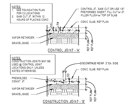
A5 TYPICAL CONTROL AND CONSTRUCTION JOINTS 3/4" x 1'-0"
