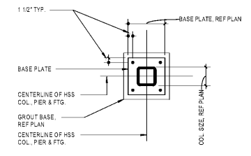
D4 TYPICAL BASE PLATE 3/4" x 1'-0"
