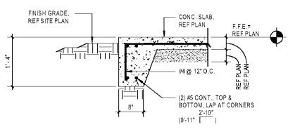
A2 TYPICAL AT EXTERIOR PATIO SLAB 3/4" x 1'-0"
