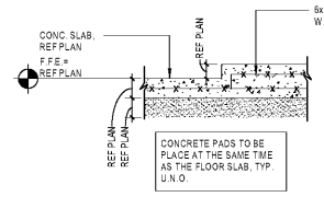
C2 TYPICAL INTEGRAL CONCRETE CURB 3/4" x 1'-0"
