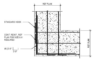
A3 TYPICAL AT CONCRETE FOOTING CORNER 3/4" x 1'-0"
