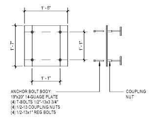
A4 TYPICAL AT SAFE BEARING PLATE 3/4" x 1'-0"
