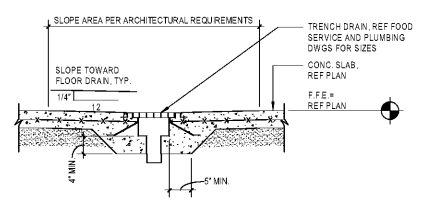
S4 TYPICAL AT INTERIOR TRENCH DRAIN 3/4" x 1'-0"
