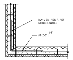
S3 TYPICAL AT 8" KNOCK-OUT BOND BEAM CORNER 3/4" x 1'-0"
