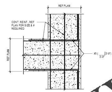
C3 TYPICAL CONCRETE FOOTING INTERSECTION 3/4" x 1'-0"
