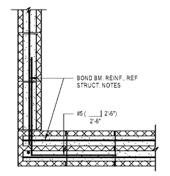
D2 MULT-DIMENSION CMU STEM WALL CORNER 3/4" x 1'-0"
