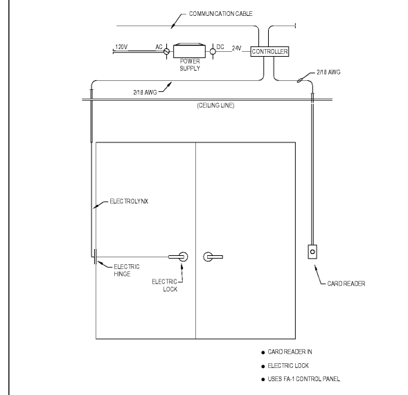
SECURITY DOOR WIRING DETAIL - LAC23 No Scale
