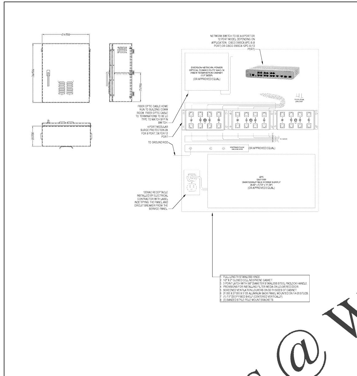
NETWORK ZONE SYSTEM ENCLOSURE No Scale
