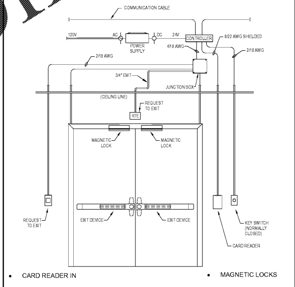
SECURITY DOOR WIRING DETAIL - LAC25 No Scale
