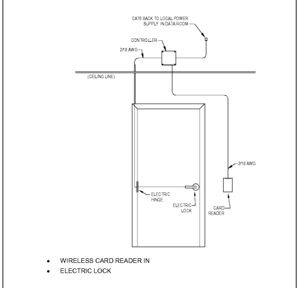
SECURITY DOOR WIRING DETAIL - POE No Scale
