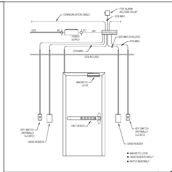
SECURITY DOOR WIRING DETAIL - LAC05 No Scale
