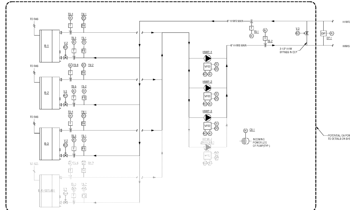
2 HOT WATER SCHEMATIC 12" = 1'-0"
