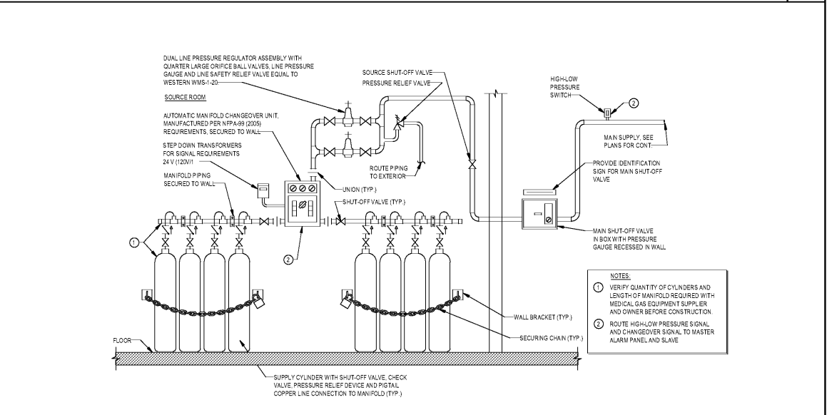
MEDICAL GAS MANIFOLD SYSTEM No Scale
