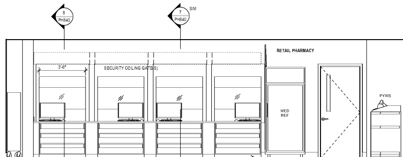
5 RETAIL PHARMACY - EAST. 3/8" = 1'-0"
