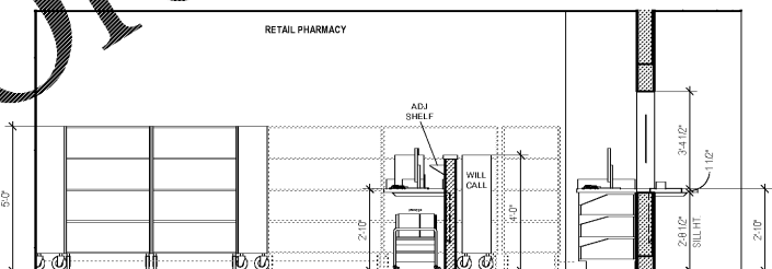
2 RETAIL PHARM. EAST AT VERIFY / REFILL 3/8" = 1'-0"
