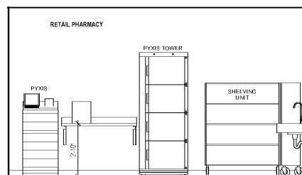
7 RETAIL PHARMACY - WEST. 3/8" = 1'-0"
