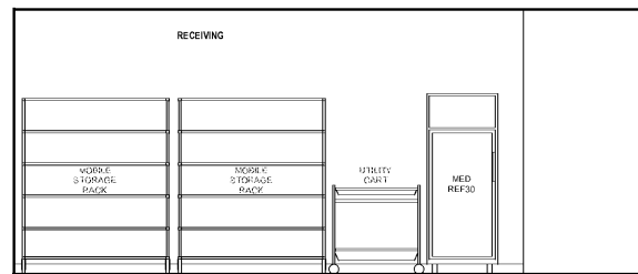
14 RETAIL PHARMACY - RECEIVING - SOUTH. 3/8" = 1'-0"
