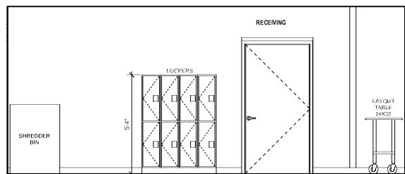
12 RETAIL PHARMACY - RECEIVING NORTH 3/8" = 1'-0"
