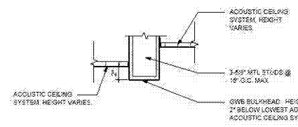
13 DETAIL BULKHEAD 1 1/2" = 1'-0"
