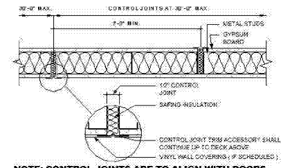
7 DETAIL CONTROL JOINTS 1 1/2" = 1'-0"
