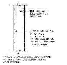
10 DETAIL BLOCKING REINFORCING 1 1/2" = 1'-0"
