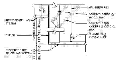
14 DETAIL SOFFIT 1 1/2" = 1'-0"
