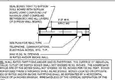
8 DETAIL ELECTRIC BOX IN RATED WALL 3/4" = 1'-0"
