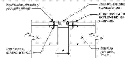
6 DETAIL WALL EXPANSION JOINT 3" = 1'-0"
