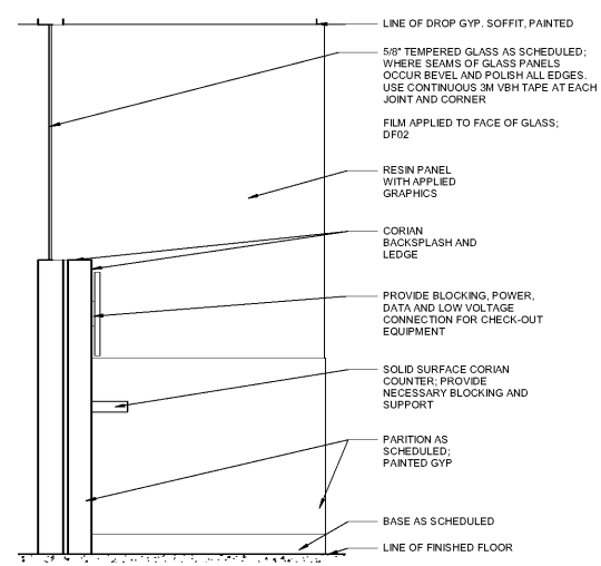
3 TYP. CHECK OUT DESK SOUTH ELEVATION DETAIL 3/4\"/>
