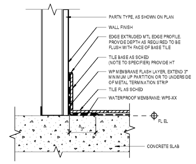
1 DETAIL AT TILE BASE 3" = 1'-0"
