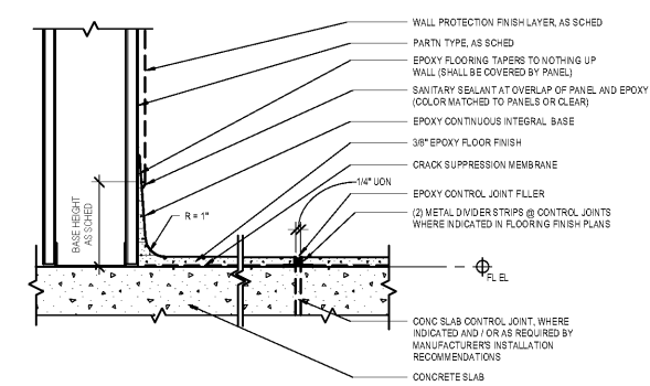
5 EPOXY FLOOR & BASE DETAIL W/WALL PROTECTION 3" = 1'-0" A920-2012A
