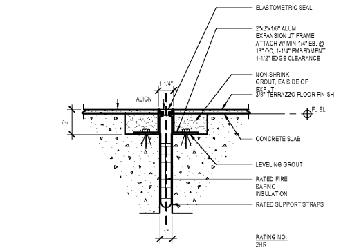
2 TERRAZZO FLOOR EXPANSION JOINT 3" = 1'-0" A975-2220C
