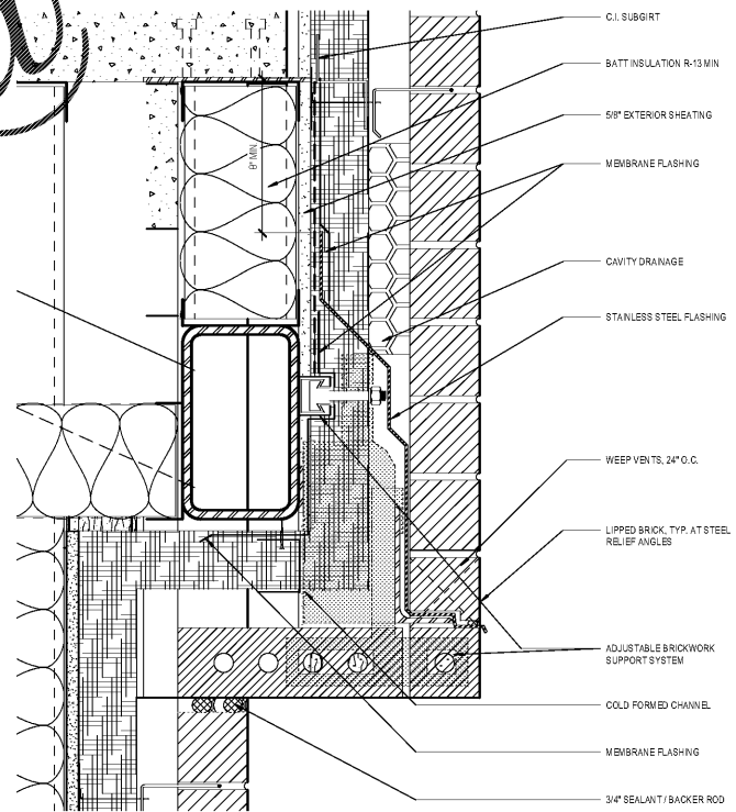
5 Enlarged TYP. Brick to Brick Lintel Support 3" = 1'-0"
