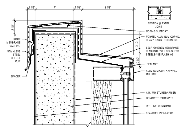
1 CW DETAIL 3" = 1'-0"
