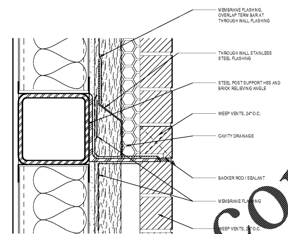
4 E.C.8 - TYP. Brick Horizontal Control Joint above Top of Slab - Callout 1 3" = 1'-0"
