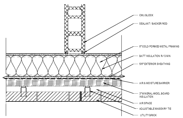
2 EXTERIOR DETAIL - PLAN 1 1/2" = 1'-0"
