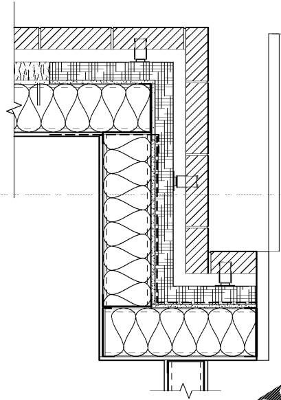
4 EXTERIOR DETAIL - PLAN 1/12\"/>
