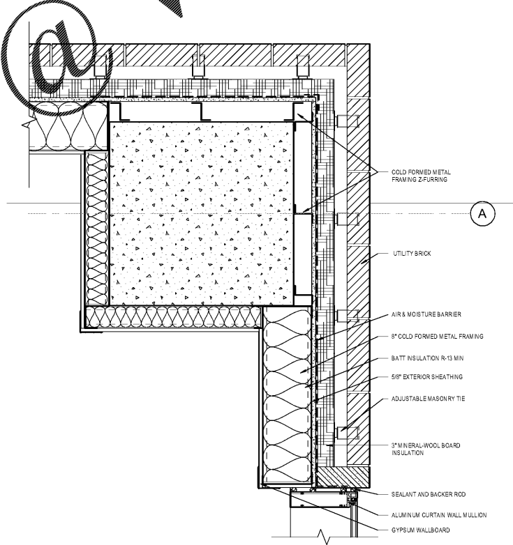
2 EXTERIOR DETAIL - PLAN 1/12\"/>
