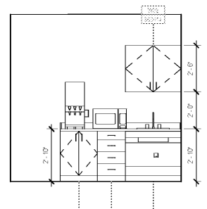
14 INFUSION NOURISHMENT ROOM - W 3/8" = 1'-0"
