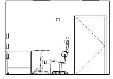
8 MAMMO DIAGNOSTIC - W 3/8" = 1'-0"
