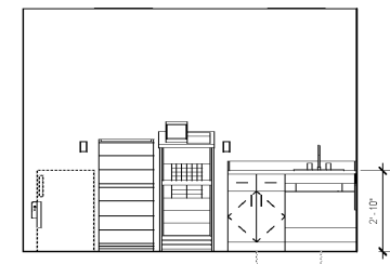
13 TYP INFUSION MEDS ROOM - E 3/8" = 1'-0"
