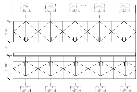
9 BREAST IMAGING TECH WORK - N 3/8" = 1'-0"
