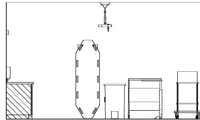
15 TYP ORTHO PROCEDURE - S 3/8" = 1'-0"
