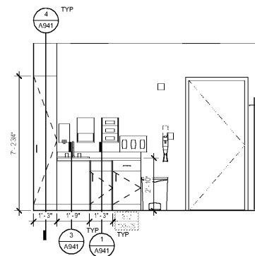
14 TYP ORTHO PROCEDURE - E 3/8" = 1'-0"
