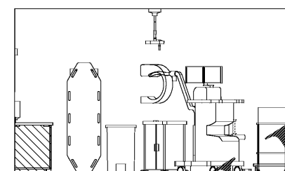
7 ORTHO PROCEDURE - S 3/8" = 1'-0"
