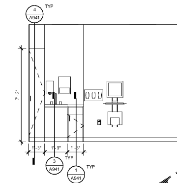
7 SPEECH THERAPY - S 3/8" = 1'-0"
