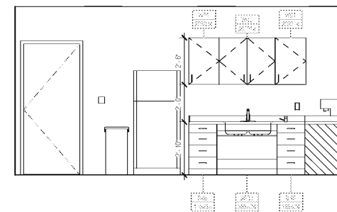
2 TPL ADL KITCHEN - S 3/8" = 1'-0"
