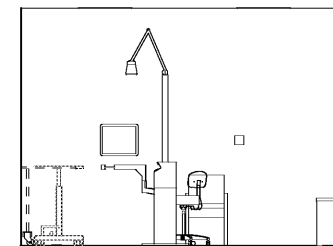
1 OPTH. TREATMENT ROOM - N 3/8" = 1'-0"
