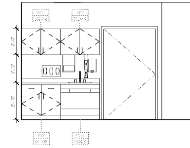
8 OPTH PROCEDURE - W 3/8" = 1'-0"
