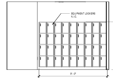
2 SECURITY WORKROOM - W 3/8" = 1'-0"
