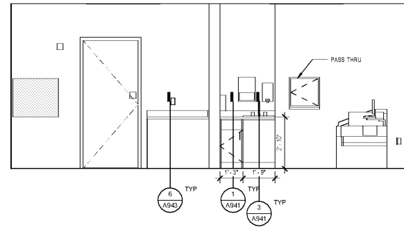
4 PAT LAB - S 3/8" = 1'-0"
