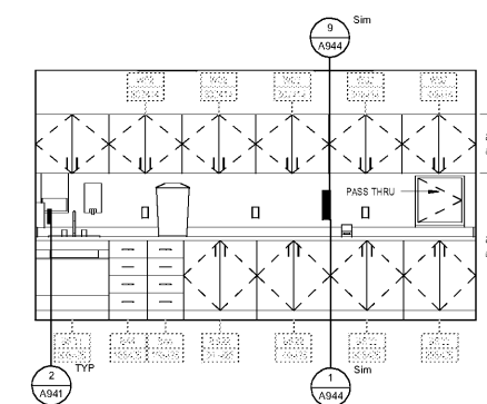
1 POC TESTING LARGE - N 3/8" = 1'-0"
