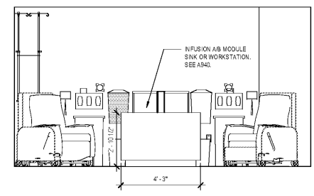
15 TYP INFUSION BAY - S 3/8" = 1'-0"
