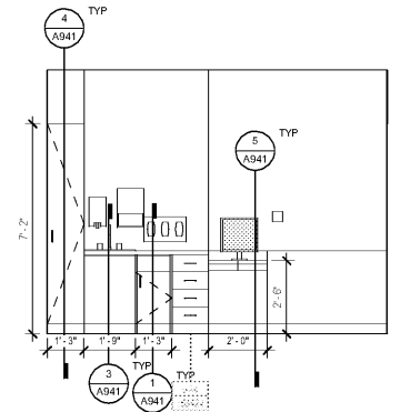
11 TYP OPHTH EXAM ROOM - S 3/8" = 1'-0"
