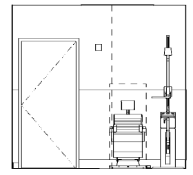
12 TYP OPHTH EXAM ROOM - W 3/8" = 1'-0"
