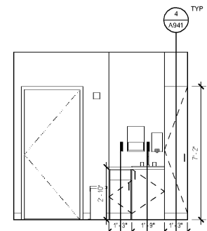
2 TYPICAL EXAM ROOM - E 3/8" = 1'-0"
