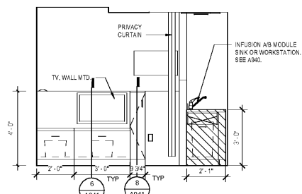
16 TYP TYO INFUSION BAY - W 3/8" = 1'-0"
