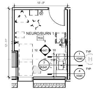
8 NEURO BURN EXAM 1/4" = 1'-0"
