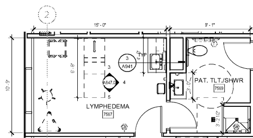
2 LYMPHEDEMA 1/4" = 1'-0"
