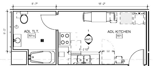
1 ADL KITCHEN 1/4" = 1'-0"
