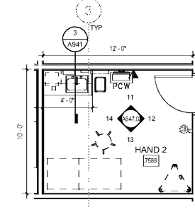
5 HAND THERAPY 1/4" = 1'-0"
