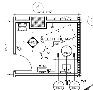
7 SPEECH THERAPY 1/4" = 1'-0"
