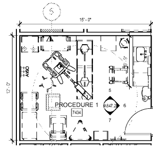
12 ORTHO PROCEDURE 1/4" = 1'-0"
