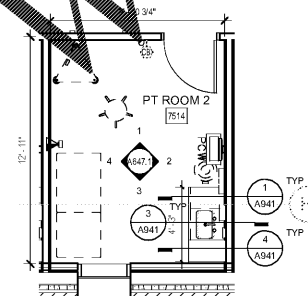
6 PT GEN EXAM 1/4" = 1'-0"
