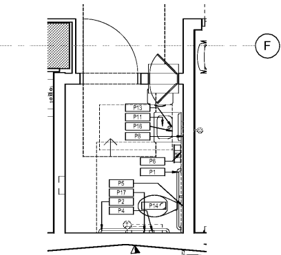
4 ENLARGED FLOOR PLAN - TYP. PACU/PREPOST RESTROOM LEVEL 5 3/8" = 1'-0"
