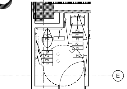
5 ENLARGED FLOOR PLAN - TYP. PUBLIC RESTROOM LEVEL 5 3/8" = 1'-0"
