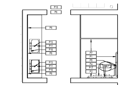
2 ENLARGED FLOOR PLAN - TYPICAL LOCKER RESTROOM LEVEL 5 3/8" = 1'-0"
