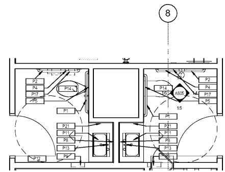
13 ENLARGED PLAN - TYP. PATIENT RESTROOM LEVEL 6,7,8 3/8" = 1'-0"
