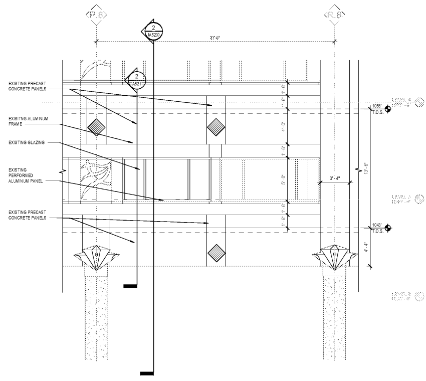
1 EXISTING GRADY ELEVATION AT LOCATION 1/4" = 1'-0"
