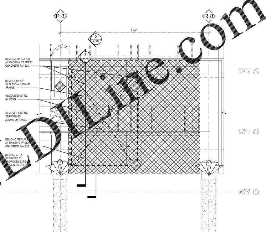
3 DEMOLITION OF NEW GRADY BRIDGE CONNECTION 1/4" = 1'-0"
