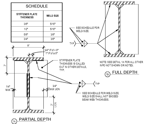
3 TYPICAL BEAM STIFFENER DETAIL 3" = 1'-0"
