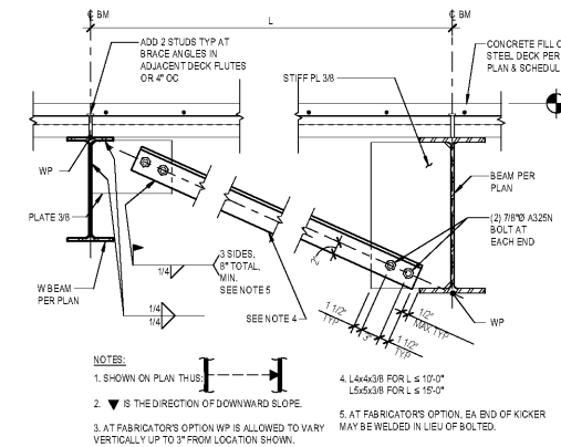
6 BOTTOM FLANGE BRACE TO BEAM 1" = 1'-0"
