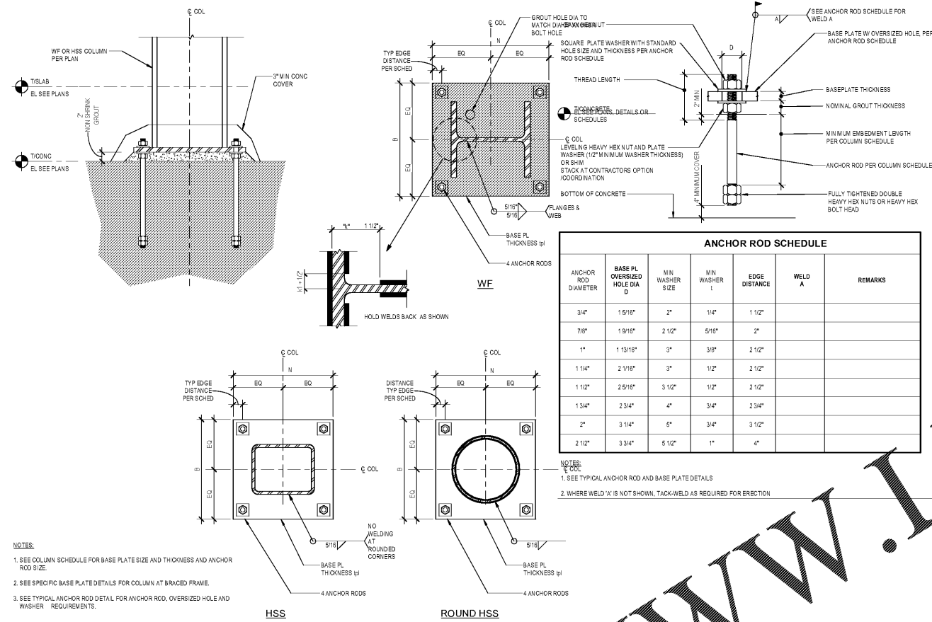
8 COLUMN BASE PLATE DETAIL 1 1/2" = 1'-0"
