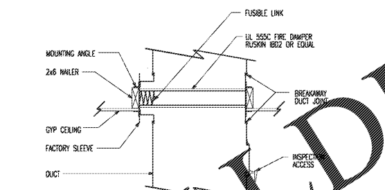
3 Horizontal Fire Damper Installation No Scale
