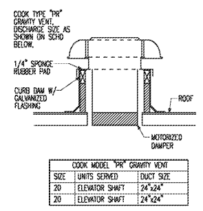
5 Exhaust Air Venting (EV-1) No Scale
