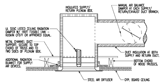
4 Ceiling Diffuser Fire Damper No Scale (Wood Truss & Cyp. Board)
