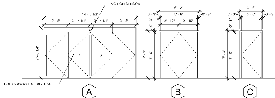
EXTERIOR DOOR ALUMINUM FRAME PAINT FINISH GLASS PANEL
