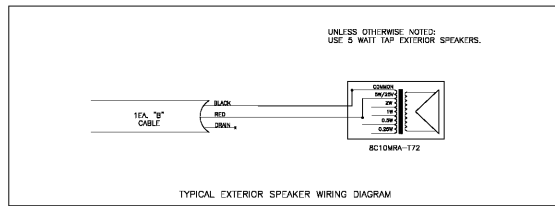
2 EXTERIOR SPEAKER WIRING DIAGRAM E5.03 NO SCALE
