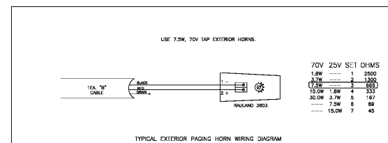
2 EXTERIOR PAGING HORN WIRING DIAGRAM E5.03 NO SCALE
