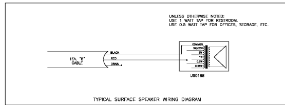
1 SURFACE SPEAKER WIRING DIAGRAM E5.03 NO SCALE
