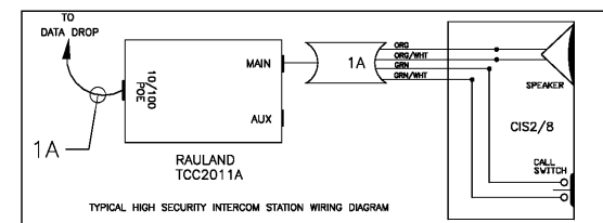
3 HIGH SECURITY INTERCOM STATION WIRING DIAGRAM E5.03 NO SCALE
