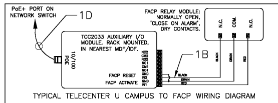
3 TELECENTER U CAMPUS TO FACP WIRING DIAGRAM E5.03 NO SCALE
