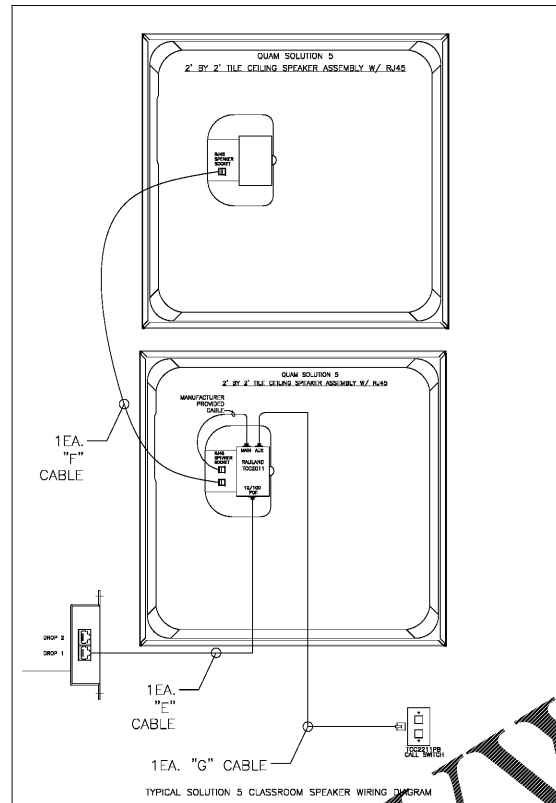
5 SOLUTION 5 SPEAKER/ CALL STATION WIRING DIAGRAM E5.03 NO SCALE
