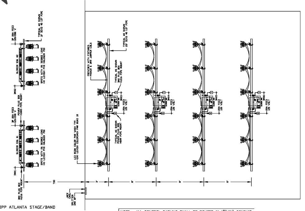
2 STAGE LIGHTING DETAIL E5.02 NO SCALE
