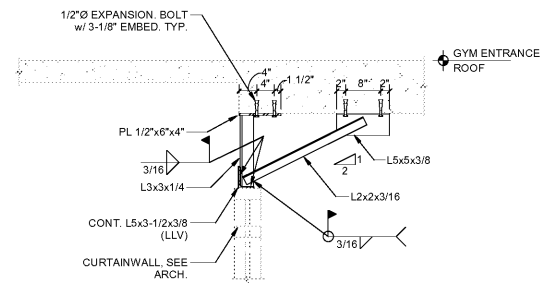
1 SECTION AT GYM ENTRANCE CURTAINWALL SCALE: 3/4" = 1'-0"
