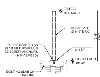
2 SECTION AT COUNTERTOP WALL SCALE: 3/4" = 1'-0"
