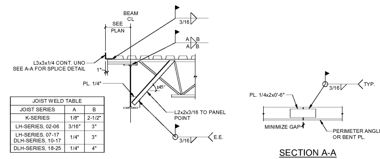
1 TYPICAL DECK PARALLEL TO EDGE BEAM (w/ JOISTS) S01-02
