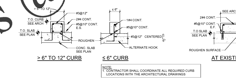
8 TYPICAL SECTION THROUGH CONCRETE CURB S01-02
