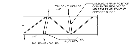
3 TYPICAL STEEL JOIST REINF. FOR CONCENTRATED LOADS S01-02
