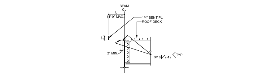
2 TYPICAL DECK PARALLEL TO EDGE BEAM (NO JOISTS) S01-02
