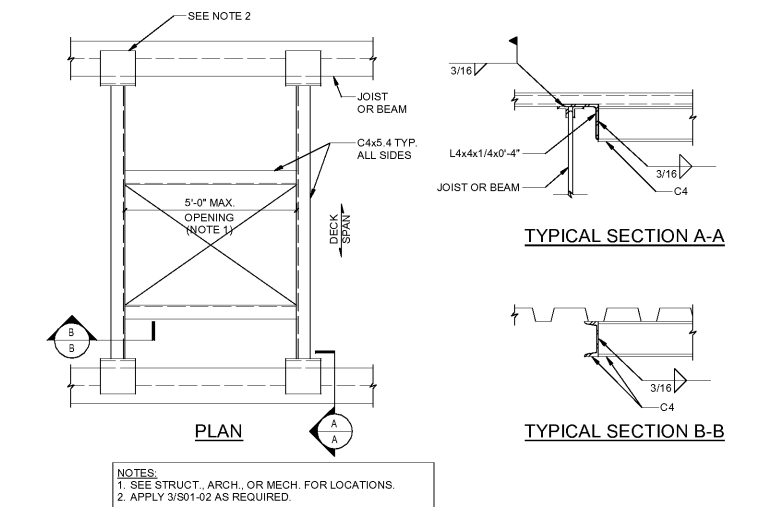
4 TYPICAL FRAMED ROOF OPENING S01-02
