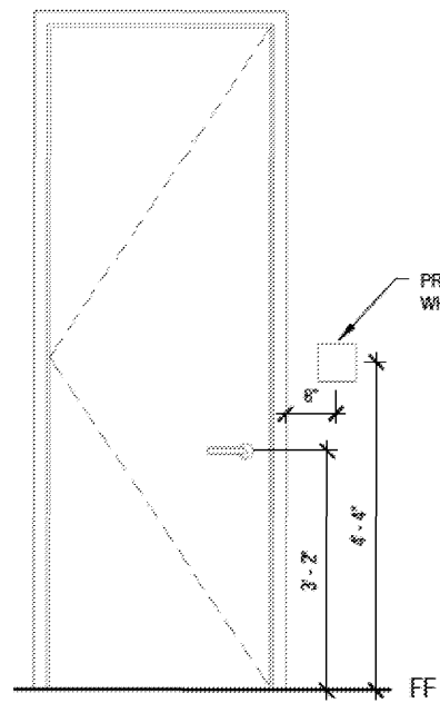
10 MOUNTING LOCATION NTS
