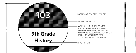
3 ROOM ID- w/ Insert Scale: Half
