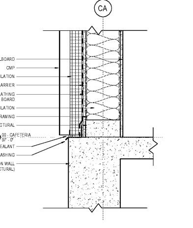
1 SILL W/ CURB AT CMP 1 1/2" = 1'-0"
