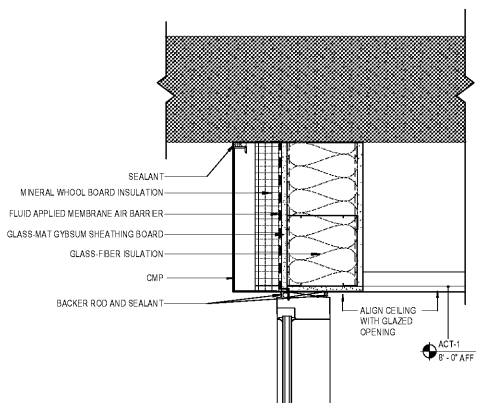
13 SF HEAD AT GYM ENTRY 1 1/2" = 1'-0"
