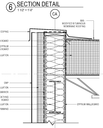
6 SECTION DETAIL 1 1/2" = 1'-0"
