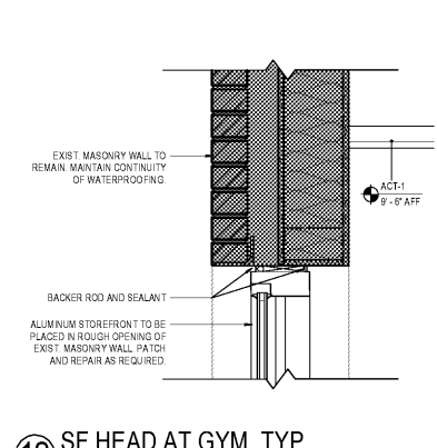
12 SF HEAD AT GYM, TYP. 1 1/2" = 1'-0"
