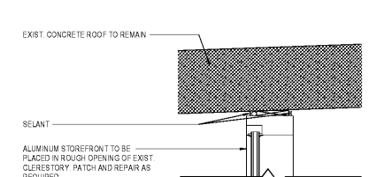
11 GYM CLERESTORY SF - HEAD, TYP. 1 1/2" = 1'-0"
