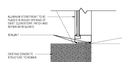
10 GYM CLERESTORY SF - SILL, TYP. 1 1/2" = 1'-0"
