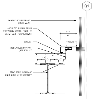
14 MEZZANINE TO EXIST. STOREFRONT, TYP. 1 1/2" = 1'-0"
