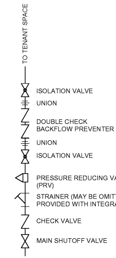
A13 P-101 TYPICAL WATER MAIN SHUTOFF DETAIL NOT TO SCALE
