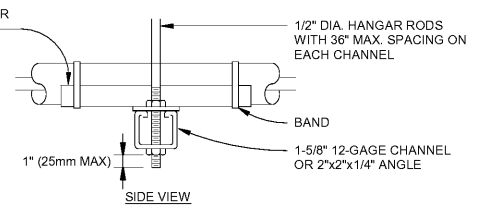
TRAPEZE HANGER FOR UP TO 1000 LB. UNIFORM LOAD
