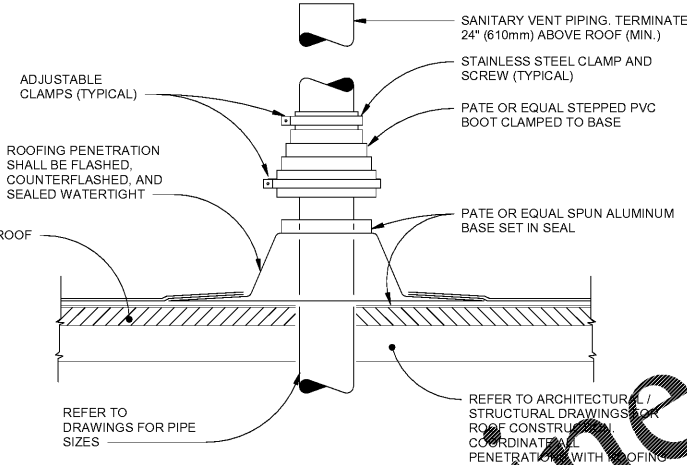
J12 P-101 TYPICAL SANITARY VENT THRU ROOF DETAIL NOT TO SCALE
