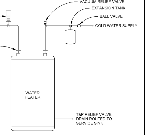
F16 P-101 TANK-TYPE HOT WATER HEATER DETAIL NOT TO SCALE
