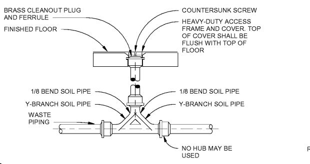
K7 P-101 TYPICAL 2-WAY EXTERIOR CLEANOUT DETAIL NOT TO SCALE
