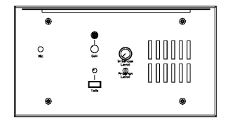
4 IC2.1 THRU 4 IC2.3 INTERCOM SPEAKER STATION 4-GANG BACK BOX RECESSED FLUSH ON WALL 48" A.F.F. BACK BOX PROVIDED AND INSTALLED BY E.C. FACEPLATE PROVIDED AND INSTALLED BY P.S.C.
