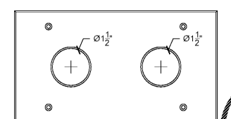
4 ST1.1 THRU 4 ST1.2 SPEAKER PASS THRU PLATE 4-GANG BACK BOX SURFACE MTD. ON CEILING BACK BOX PROVIDED AND INSTALLED BY E.C. FACEPLATE PROVIDED AND INSTALLED BY P.S.C.
