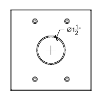
2 CAM1.1 CAMERA I/O PLATE 2-GANG BACK BOX RECESSED FLUSH ABOVE CTRL. BOOTH WINDOW BACK BOX PROVIDED AND INSTALLED BY E.C. FACEPLATE PROVIDED AND INSTALLED BY P.S.C.
