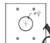
2 VM2.1 THRU 2 VM2.2 VIDEO MONITOR I/O PLATE 2-GANG BACK BOX RECESSED FLUSH ON WALL 72" A.F.F. BACK BOX PROVIDED AND INSTALLED BY E.C. FACEPLATE PROVIDED AND INSTALLED BY P.S.C.
