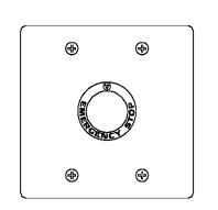
2 ES1.1 EMERGENCY STOP STATION 2-GANG BACKBOX RECESSED FLUSH ON WALL 48" A.F.F. BACKBOX PROVIDED AND INSTALLED BY E.C. FACEPLATE PROVIDED AND INSTALLED BY P.S.C.
