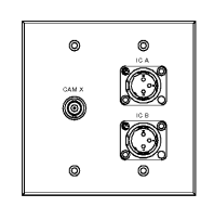
2 CAM2.1 THRU 2 CAM2.6 CAMERA TIE-LINE & INTERCOM PLATE 2-GANG BACK BOX RECESSED FLUSH ON WALL 18" A.F.F. BACK BOX PROVIDED AND INSTALLED BY E.C. FACEPLATE PROVIDED AND INSTALLED BY P.S.C.
