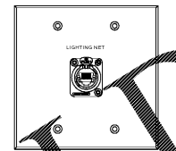
2 LN2.1 THRU 2 LN2.4 LIGHTING NETWORK / DMX PLATE 2-GANG BACK BOX SURFACE MTD. ON CEILING STRUCTURE BACK BOX PROVIDED AND INSTALLED BY E.C. FACEPLATE PROVIDED AND INSTALLED BY P.S.C.
