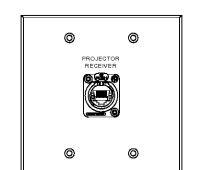
2 P1.1 PROJECTOR I/O PLATE 2-GANG BACK BOX RECESSED FLUSH ON WALL 13'-10" A.F.F. BACK BOX PROVIDED AND INSTALLED BY E.C. FACEPLATE PROVIDED AND INSTALLED BY P.S.C.
